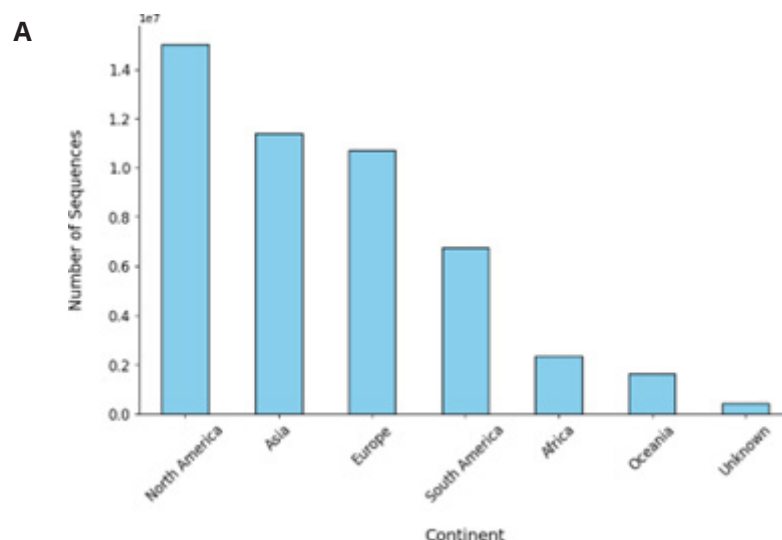
Figure 1. Global representation of African genomics in public data repositories.
