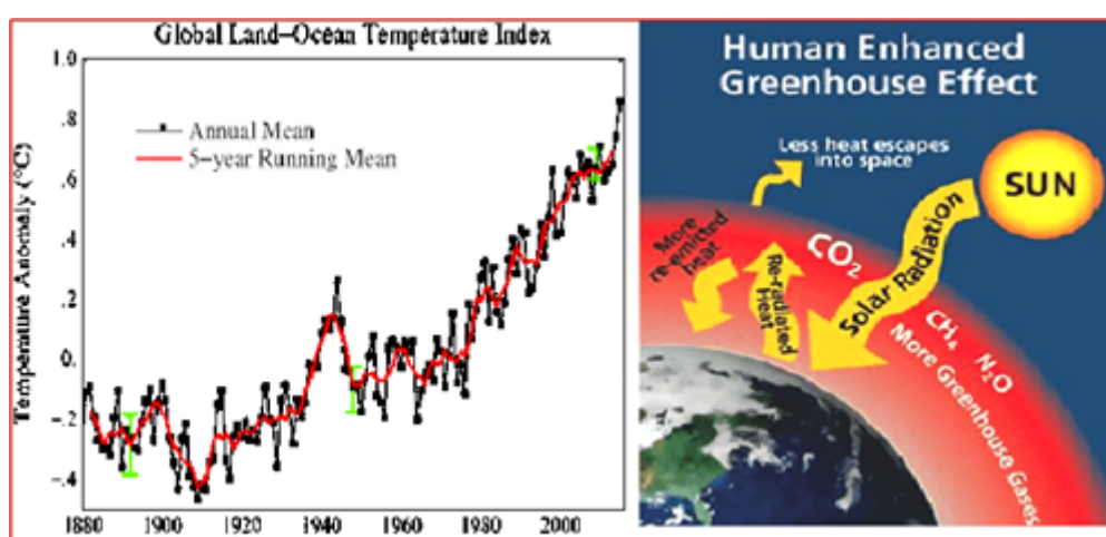
Figure 1 and 2. Global land-ocean temperature index and Greenhouse effect.
