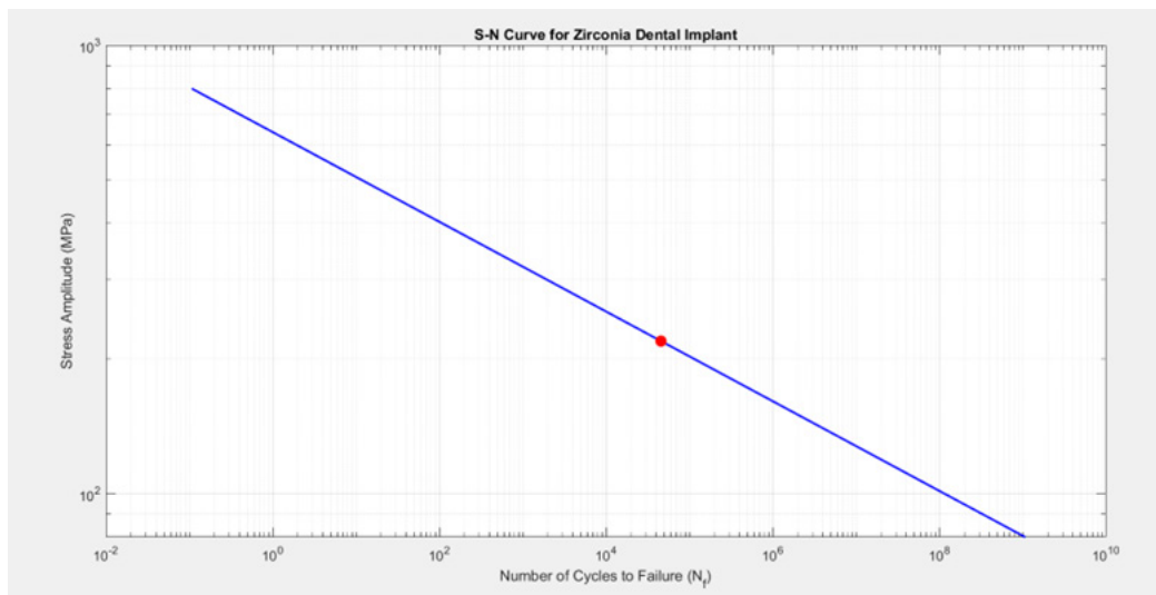
Figure 8. S-N Curve Zirconia Dental Implant.
