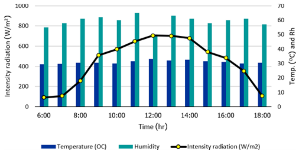
Figure 3. Relationship of time to solar radiation intensity, temperature and relative humidity.
