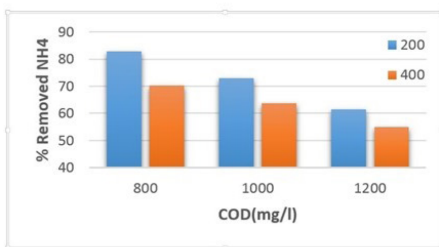
Figure 3. Ammonia removal efficiency in relation to varying inlet COD concentrations, maintaining a 24-hour retention time and 10 g/l salt concentration.
