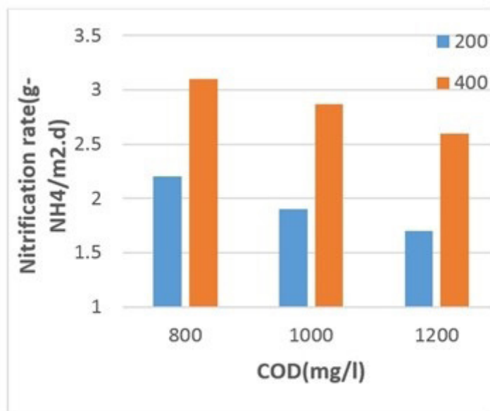
Figure 12. Nitrification velocity in relation to varying inlet COD and ammonia levels, employing a 12-hour retention time and 12 g/l salt concentration
