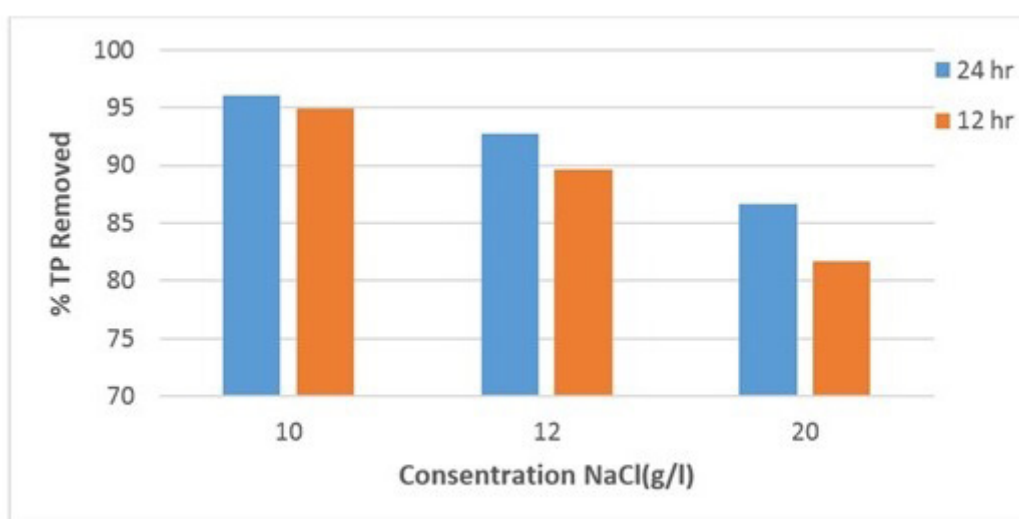
Figure 15. the total phosphorus removal efficiency under various salt concentrations and retention times.
