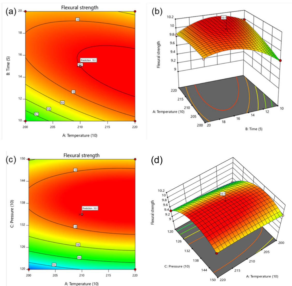
Figure 4. Surface Response Diagrams 2D, 3D illustrates the influence of interaction between mixing temperature, mixing time, and compression force on the flexural strength of tiles.
