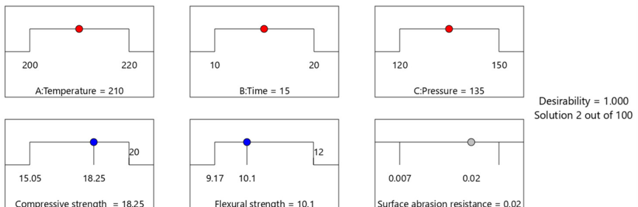
Figure 6. Optimal conditions and predicted physical properties of tiles.
