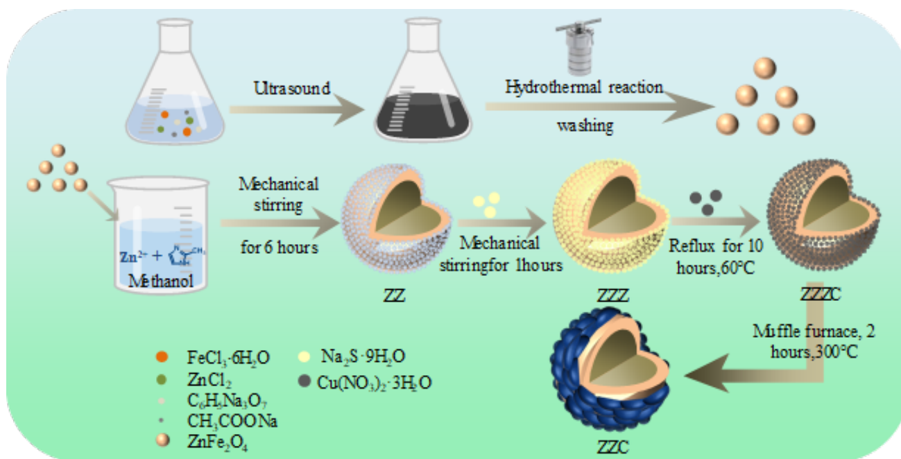
Fig. 1. Schematic showing the synthesis of the nano- ZZC complexes.
