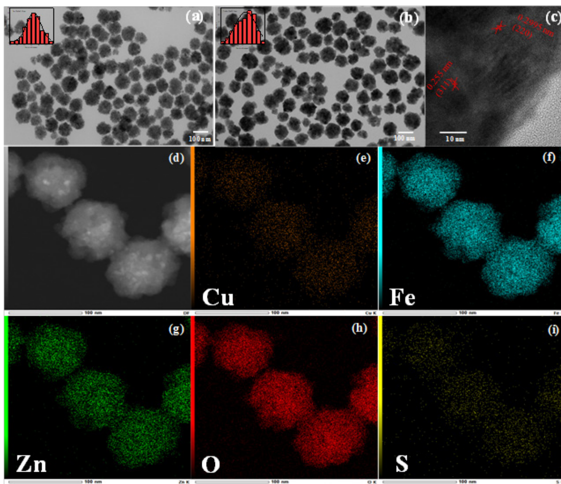
Fig. 2. TEM image of ZnFe 2 O 4 (a) and ZFC composites (b). HRTEM of nano-ZFC composites (c). Images of EDS element mapping of nano-ZFC composites (d, e, f, g, h, i)
