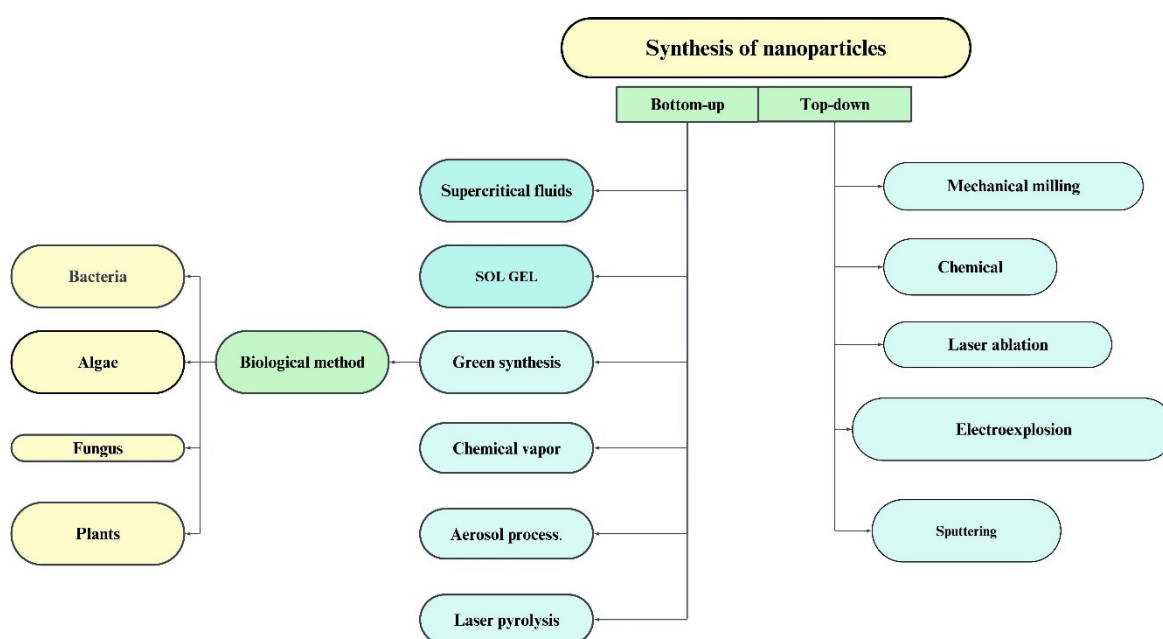
Figure 4. Nanoparticle synthesis
