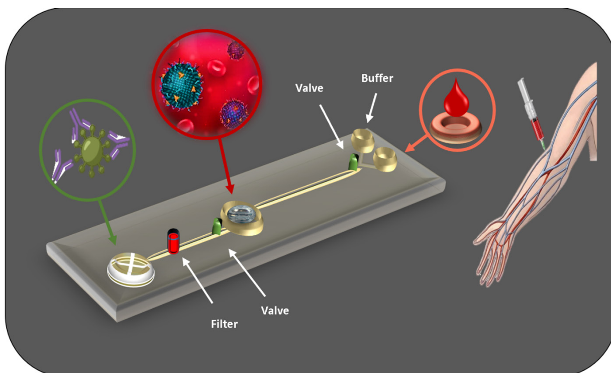
Schem1: The schematic diagram of herpes virus detection by microfluidic devices
