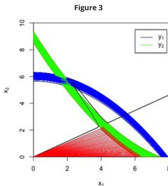
Figure 3 : Fit of two models represented in blue and green curves. Defining the tolerable region under the fitted model by the red lines, which partition the area to calculate the A_{\text{TR}^{(m)}} .
