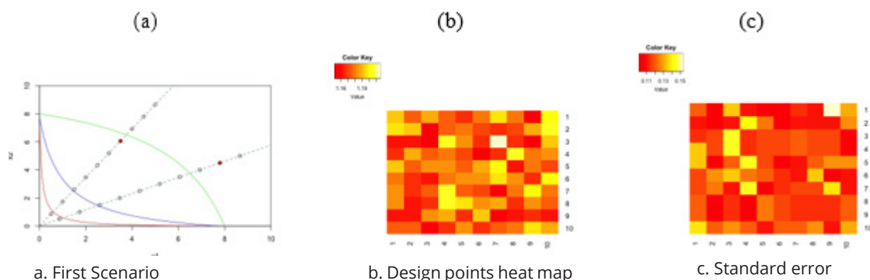
Figure 11: Panel (a) represents the 1st Scenario for second case with ray plot and the BOFED point at ( x_1 = 7 , x_2 = 9 ). Panel (b) shows the first scenario heat map of the possible design points and Panel (c) shows the Standard error around all possible design points.
