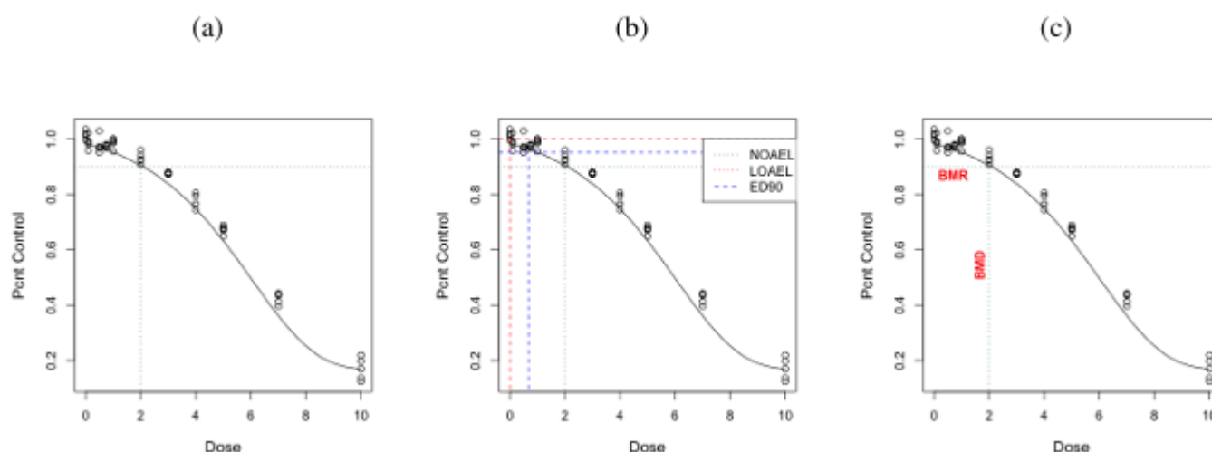
Figure 1: The dose-response model is fitted to simulated data by the solid line. The region of the tolerable dose is bounded by the percent to control vertically at ED 90 and the chemical dose horizontally at two dose, presented by dashed green lines in panel (a). NOAEL, LOAEL and ED 90 are introduced in panel (b), in red, blue and green dashed lines respectively. BMD and BMR are explained in panel (c), where the bounded rectangle area represents the tolerable region; this shows the safest dose at 10% reduction in the percent to control.
