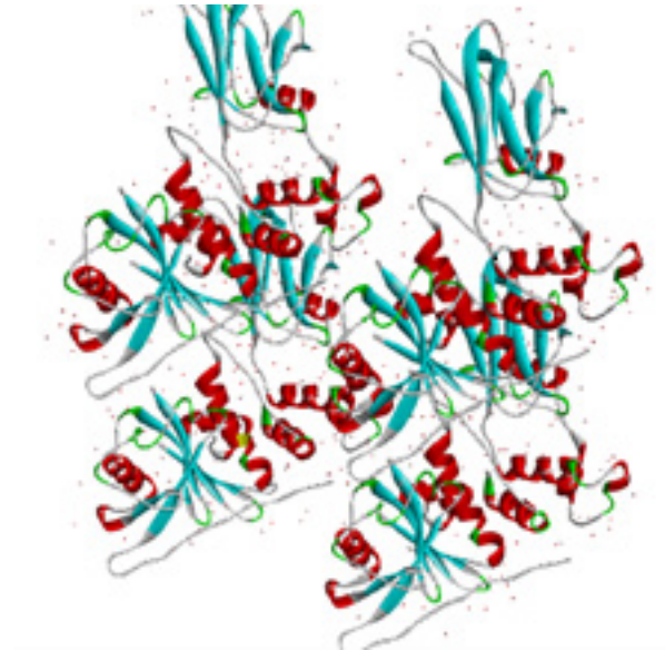
Figure 2: Crystal Structure of VHL Tumor Suppressor Protein.
