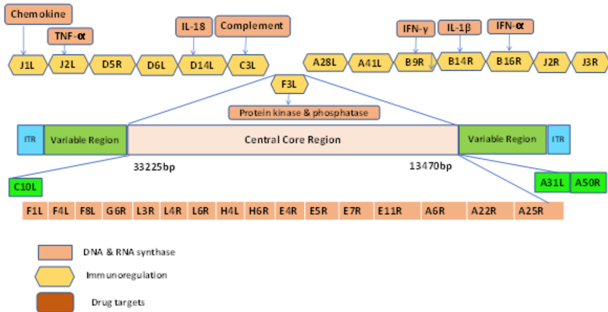
Figure 2. Genome Structure &amp; Potential antiviral targets of MPXV
