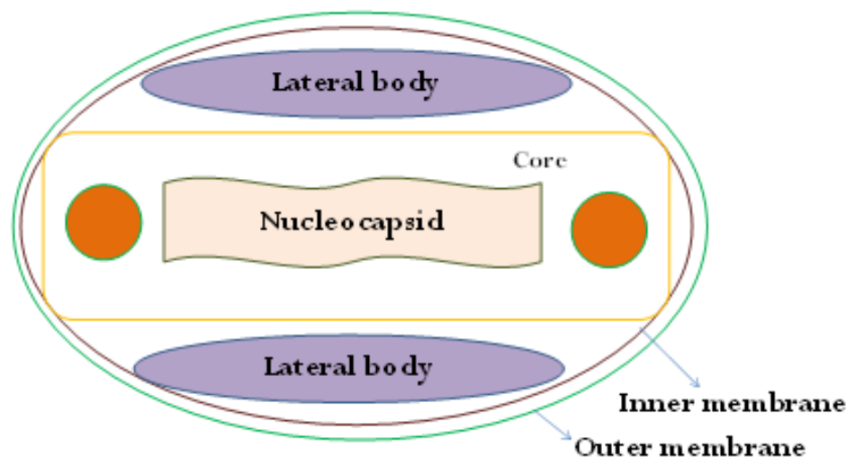
Figure 1. Structure of Monkeypox
